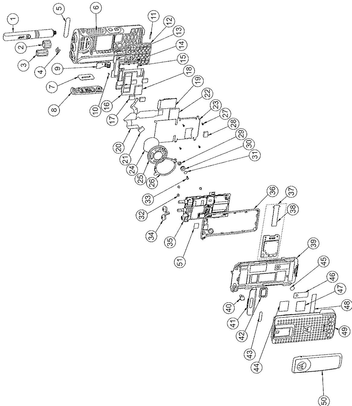
Figure 5-30. Full Keypad Model Exploded View
